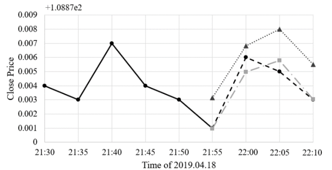
Fig. 3. The effect of the ARIMA model
